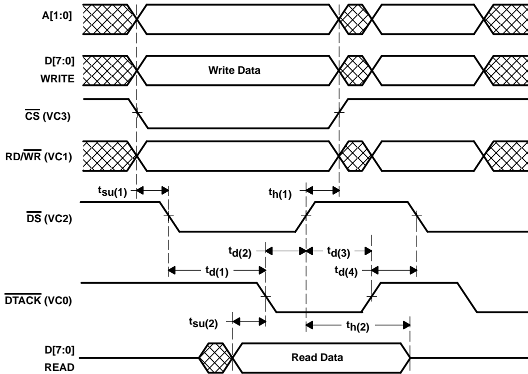
Figure 3–3. Parallel Host Interface A Timing
