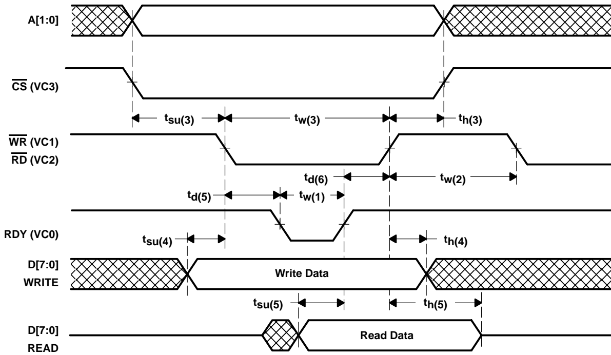
Figure 3–4. Parallel Host Interface B Timing
