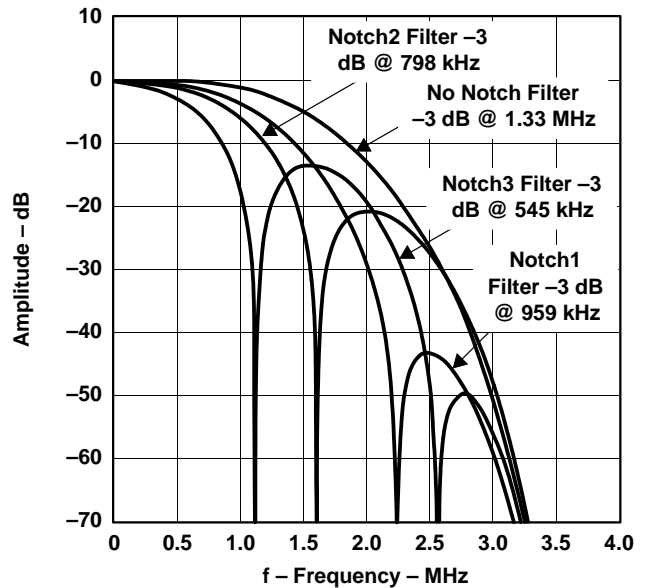
Figure 2–8. Color Low-Pass Filter With Notch Filter Response (PAL Square Pixel Sampling)
