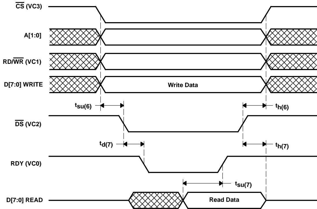
Figure 3–5. Parallel Host Interface C Timing
