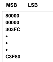
Figure 4–1. TVP5031 Microcode in Hex-ASCII Format
