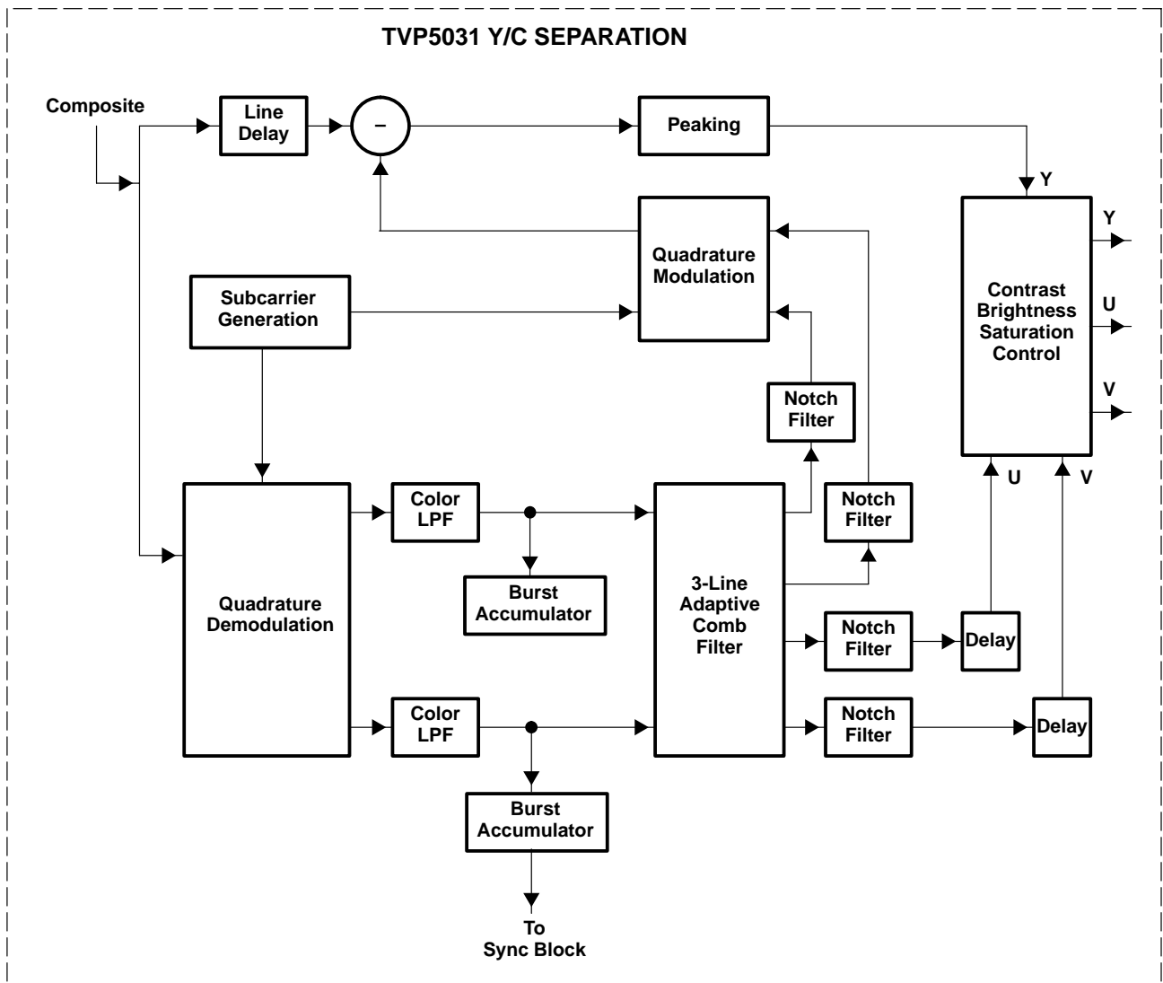
Figure 2–4. Y/C Separation Block Diagram
