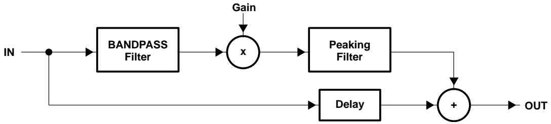
Figure 2-14. Luminance Edge-Enhancer Peaking Block Diagram
