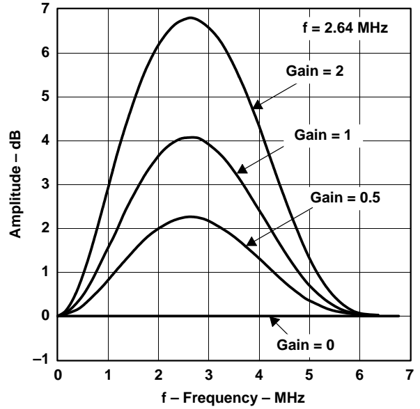
Figure 2-16. Peaking Filter Response, 13.5 MHz Sampling Rate
