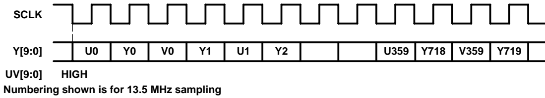
Figure 2–23. 10-Bit 4:2:2 Output Format
