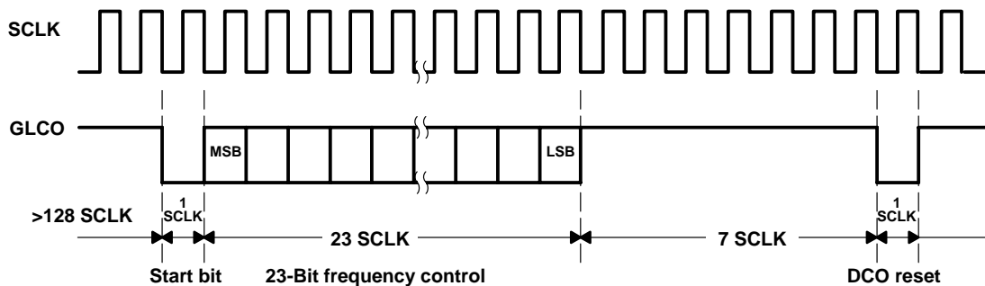
Figure 2–20. GLCO Timing
